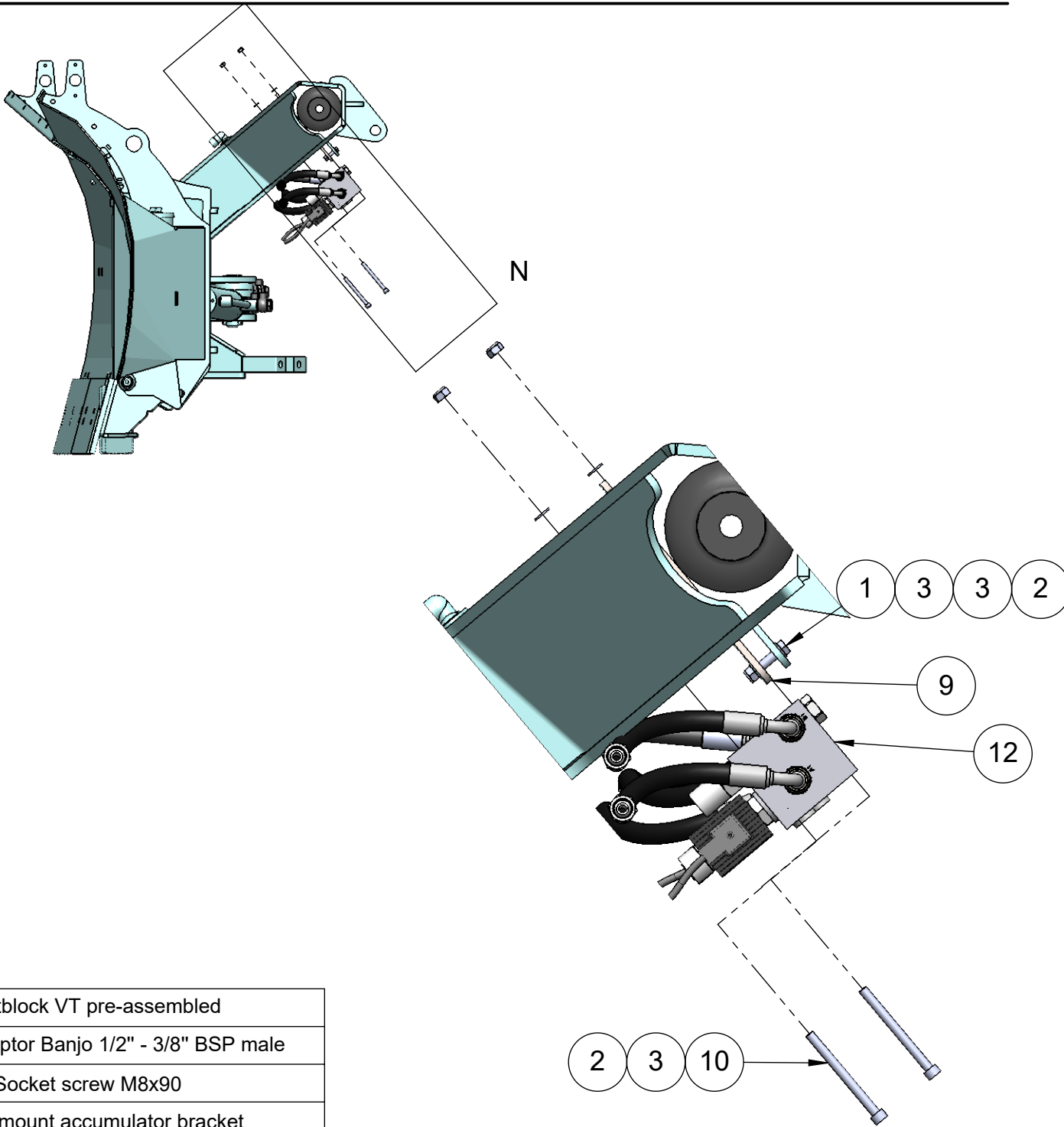
DETAIL N SCALE 1 : 5
